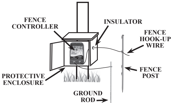
Diagram 4. Outdoor Installation
